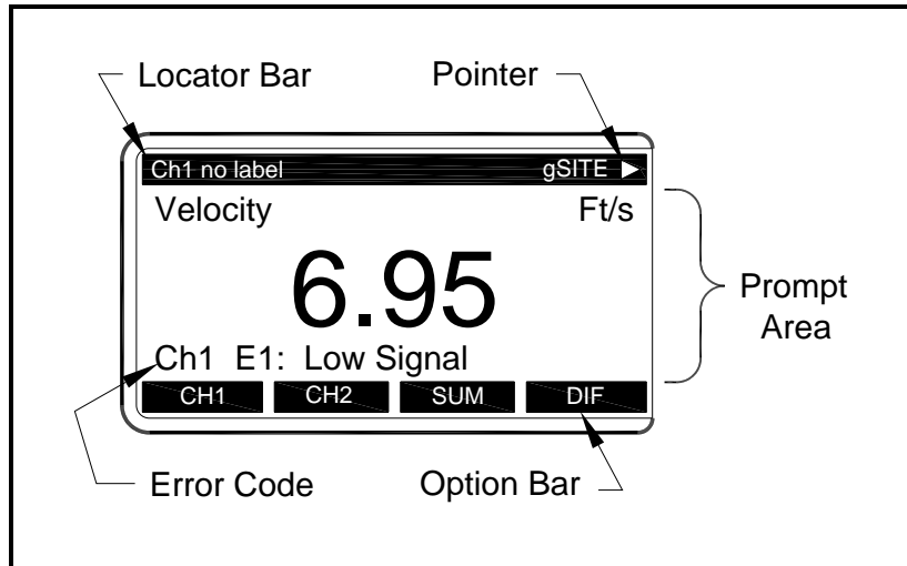
Figure 3-2: Display Screen Components
