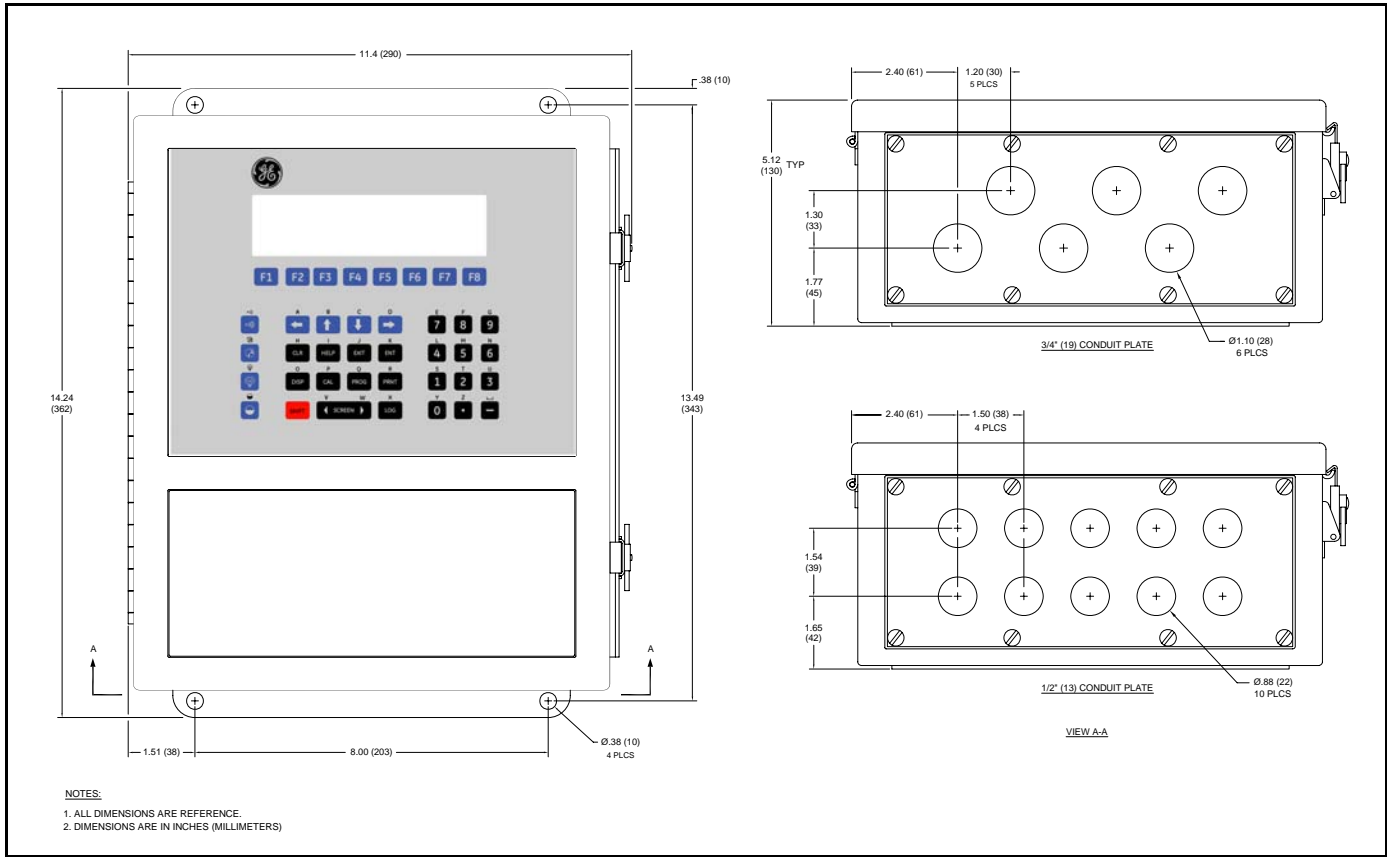
Figure 1-5: Model GM868 Type 4X Enclosure (ref. dwg # 712-1056)
