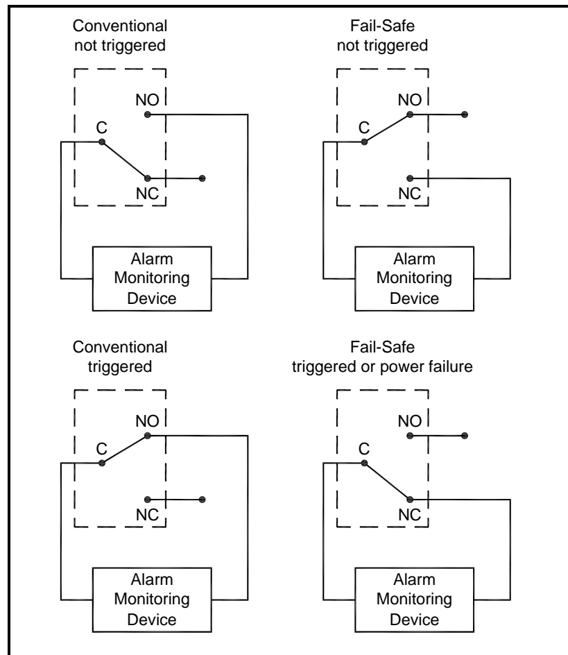
Figure 1-6: Conventional and Fail-Safe Operation
