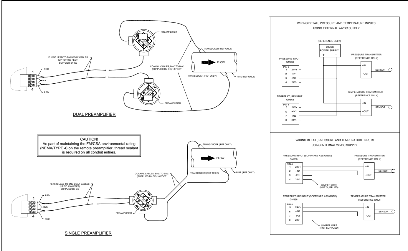
Figure 1-1-1: Model GM868 Transducer Wiring (ref. dwg #702-213, sht 2)
