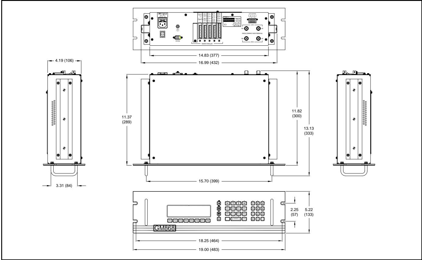
Figure C-1: Model GM868 Rack Mount Enclosure (ref. dwg #712-1078)
