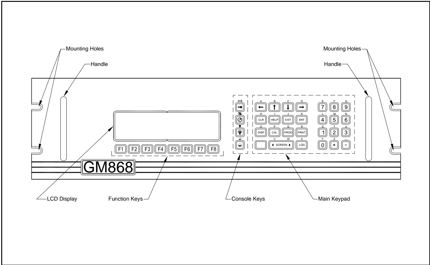
Figure C-3: Model GM868 Rack Mount Enclosure - Front Panel Layout
