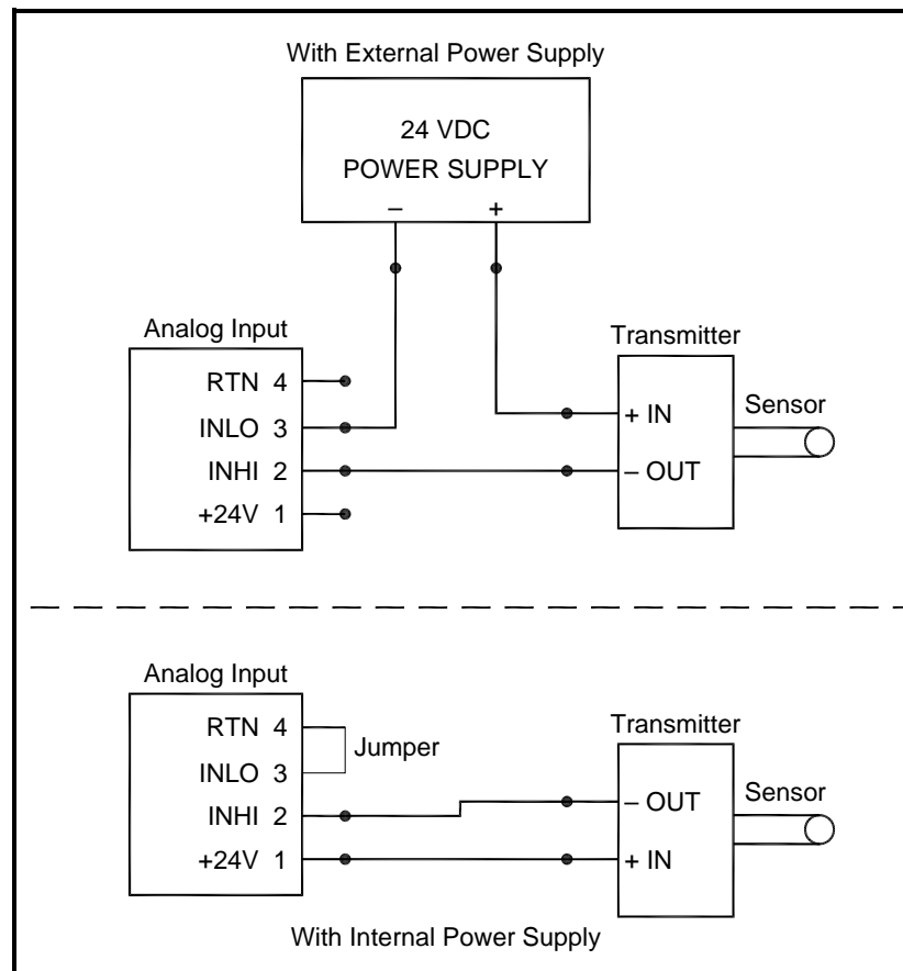
Figure 1-7: Analog Input Wiring Diagram
