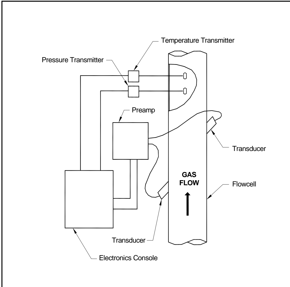
Figure 1-1: A Typical Model GM868 System
