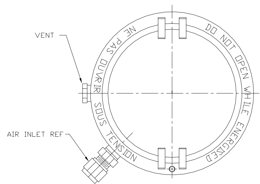
VIEW A-A SCALE NONE
